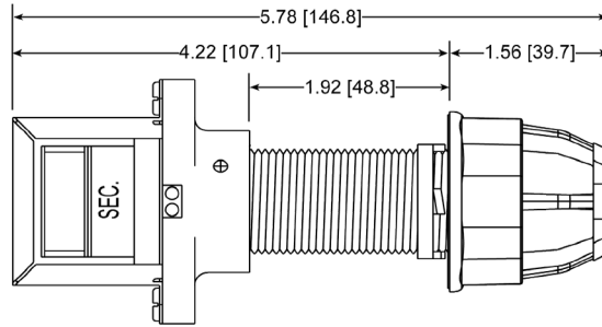
Long Barrel
